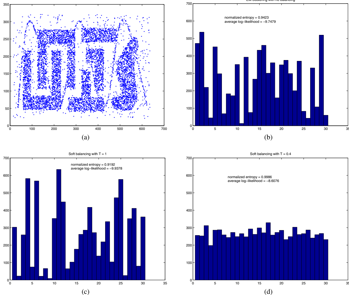
Figure 2. Balanced clustering results on t4 dataset: (a) t4 dataset; histogram distribution of cluster sizes when clustering t4 into 30 groups using (b) EM clustering with spherical Gaussian models and no balancing; (c) mixture-of-spherical Gaussians clustering with soft balancing ( T=1 ); (d) mixture-of-spherical Gaussians clustering with soft balancing ( T=0.4 ).
