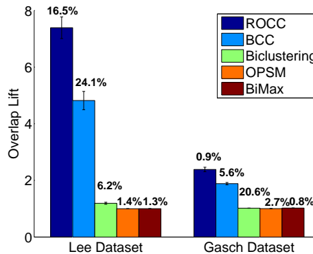
Figure 5. Comparison of ROCC with other co-clustering algorithms on the Lee and Gasch datasets. The number above each bar indicates the percentage of the data matrix entries clustered by each algorithm.
